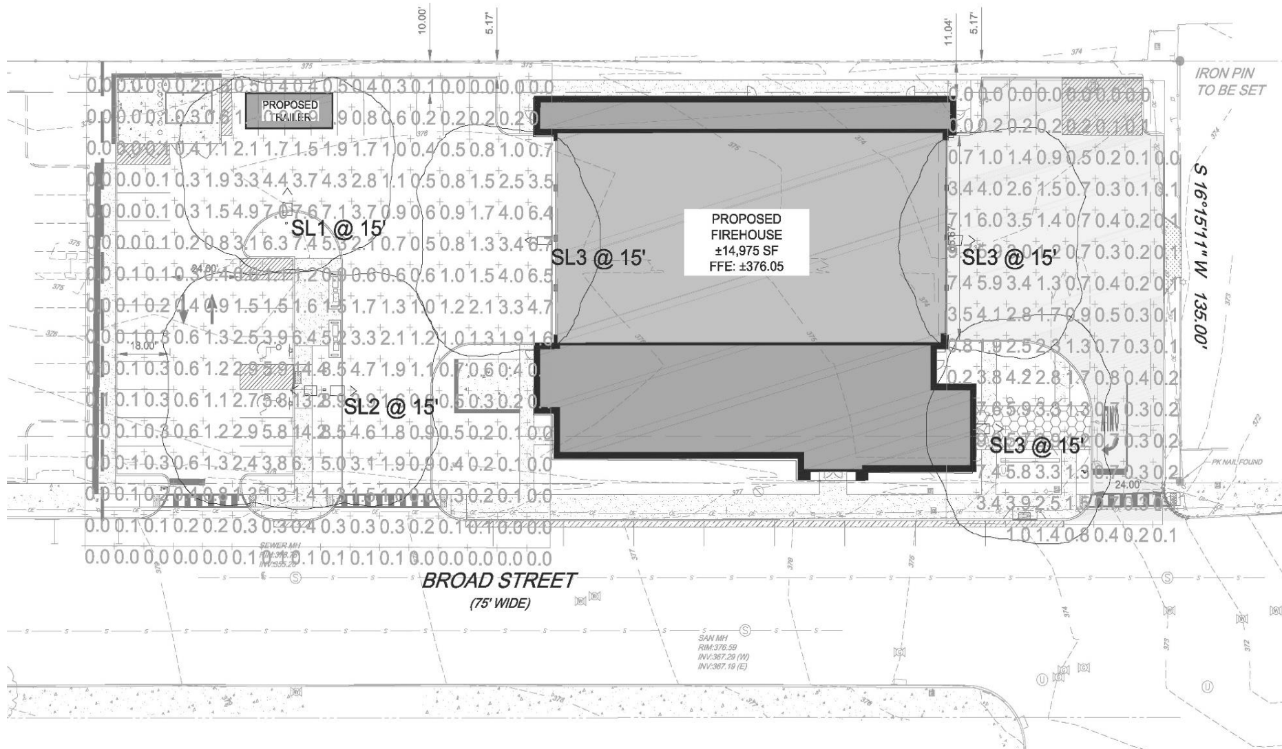
SITE LIGHTING PLAN
